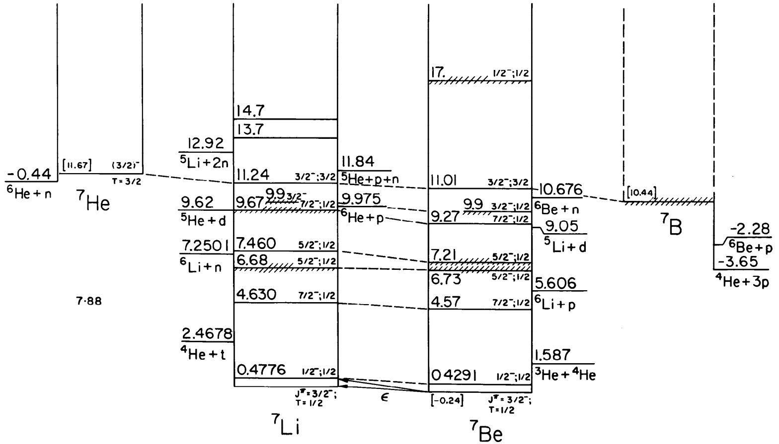
Fig. 3: Isobar diagram, A = 7 . The diagrams for individual isobars have been shifted vertically to eliminate the neutron-proton mass difference and the Coulomb energy, taken as E_C = 0.60Z(Z-1)/A^{1/3} . Energies in square brackets represent the (approximate) nuclear energy, E_N = M(Z, A) - ZM(\text{H}) - NM(\text{n}) - E_C , minus the corresponding quantity for {}^7\text{Li} : here M represents the atomic mass excess in MeV. Levels which are presumed to be isospin multiplets are connected by dashed lines.
