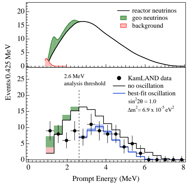
FIG. 5: Upper panel: Expected reactor \bar{\nu}_e energy spectrum along with \bar{\nu}_{geo} (model Ia of [9]) and background. Lower panel: Energy spectrum of the observed prompt events (solid circles with error bars), along with the expected no oscillation spectrum (upper histogram, with \bar{\nu}_{geo} and background shown) and best fit (lower histogram) including neutrino oscillations. The shaded band indicates the systematic error in the best-fit spectrum. The vertical dashed line corresponds to the analysis threshold at 2.6 MeV.
