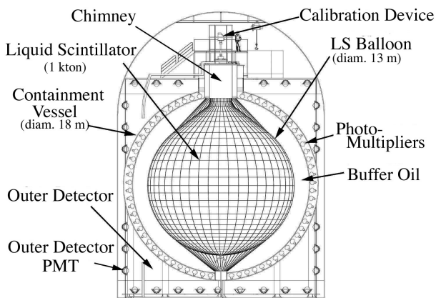
FIG. 1: Schematic diagram of the KamLAND detector.
