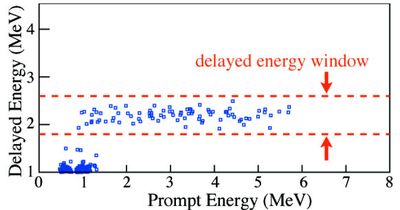
FIG. 3: Distribution of \bar{\nu}_e candidates after fiducial volume, time, vertex correlation, and spallation cuts are applied. For \bar{\nu}_e events the prompt energy is attributed to positrons and the delayed energy to neutron capture. Events within the horizontal lines bracketing the delayed energy of 2.2 MeV are consistent with thermal neutron capture on protons.
