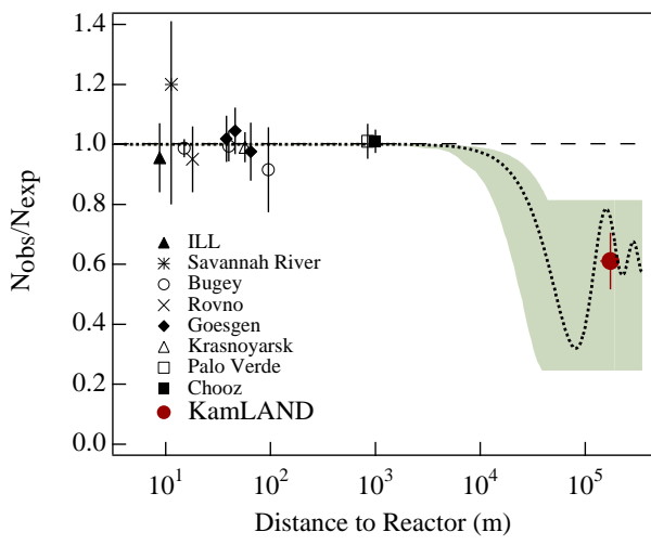
FIG. 4: The ratio of measured to expected \bar{\nu}_e flux from reactor experiments [15]. The solid circle is the KamLAND result plotted at a flux-weighted average distance of \sim 180 km. The shaded region indicates the range of flux predictions corresponding to the 95% C.L. LMA region from a global analysis of the solar neutrino data [17]. The dotted curve, \sin^2 2\theta = 0.833 and \Delta m^2 = 5.5 \times 10^{-5} \text{ eV}^2 [17], is representative of a best-fit LMA prediction and the dashed curve is expected for no oscillations.
